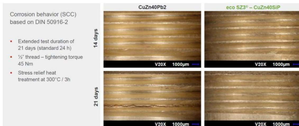
Figure 5-4: ECO SZ3 stress corrosion cracking test (DIN 50916-2) and dezincification (ISO 6509)
