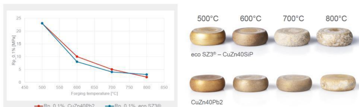
Figure 5-6: ECO SZ3 hot forming test by means of hot compression tests
