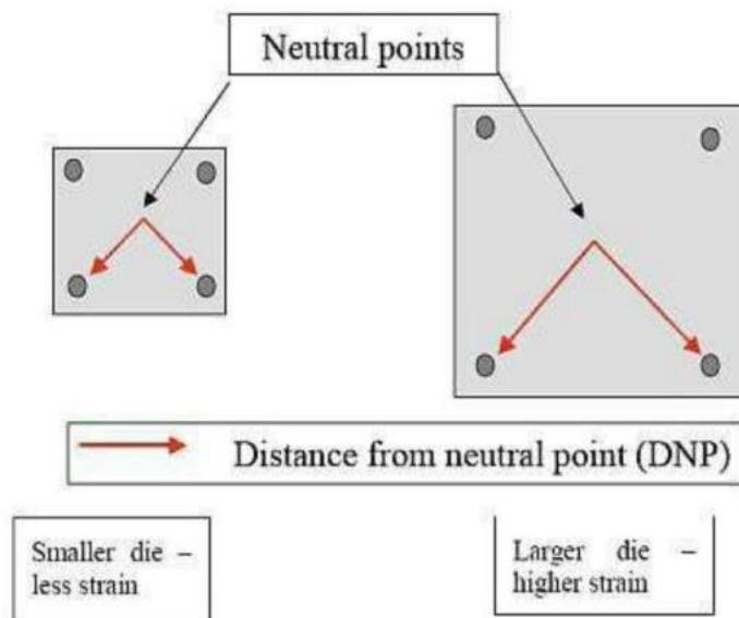
Figure 7-3: Increased thermomechanical stress in larger die FCPs
